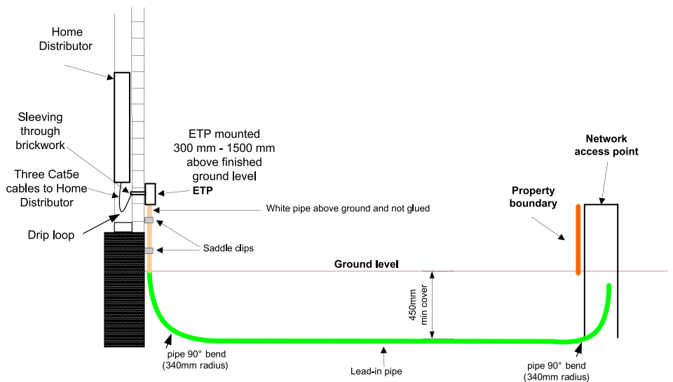
Fig 1. CROSS SECTIONAL VIEW OF A LEAD-IN INSTALLATION
