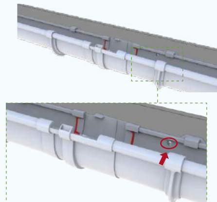
When expansion outlet and expansion joiner are used on the same run, also screw spouting adjacent to expansion joiner (refer to 2B above)
