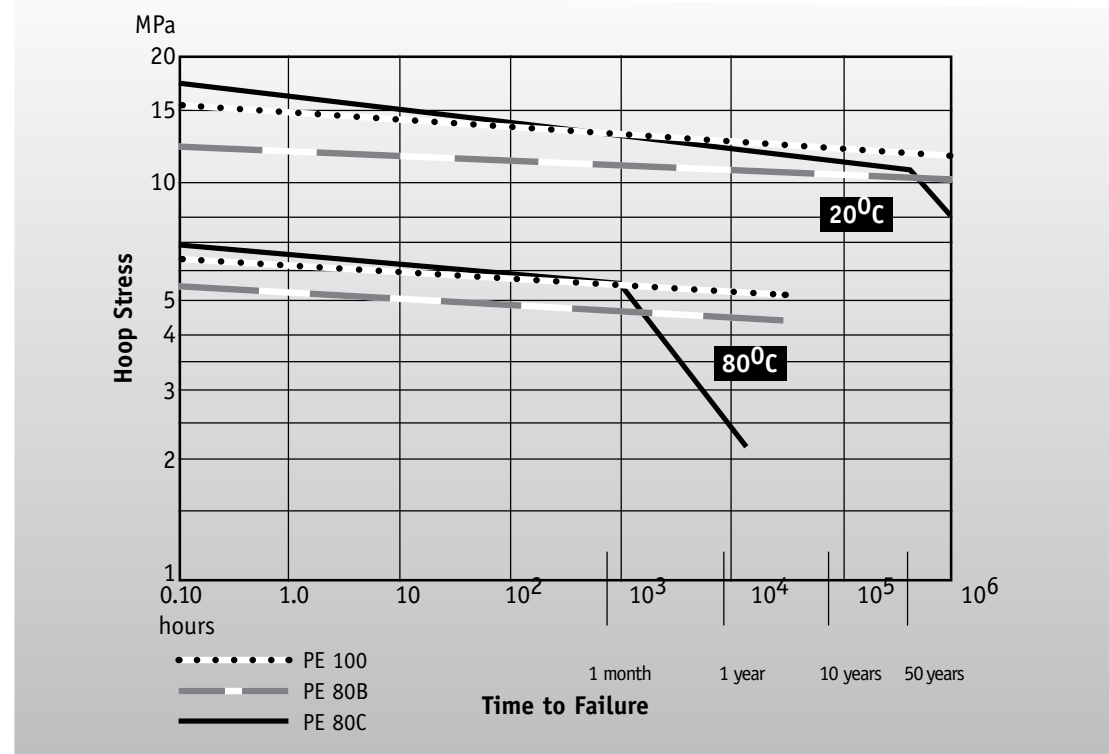
TYPICAL STRESS REGRESSION CURVES FOR MDPE
